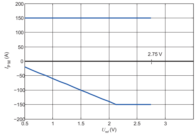
Figure 33: Measuring range versus external U_{ref} LPSR 50 A
