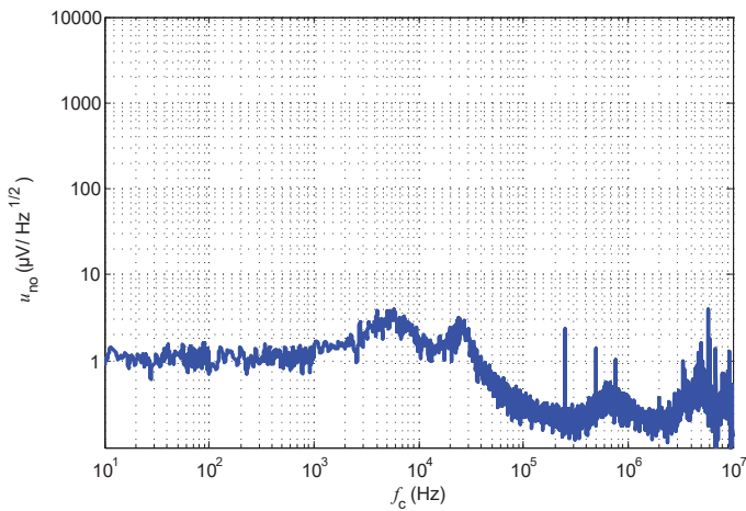
Figure 19: Noise voltage spectral density
