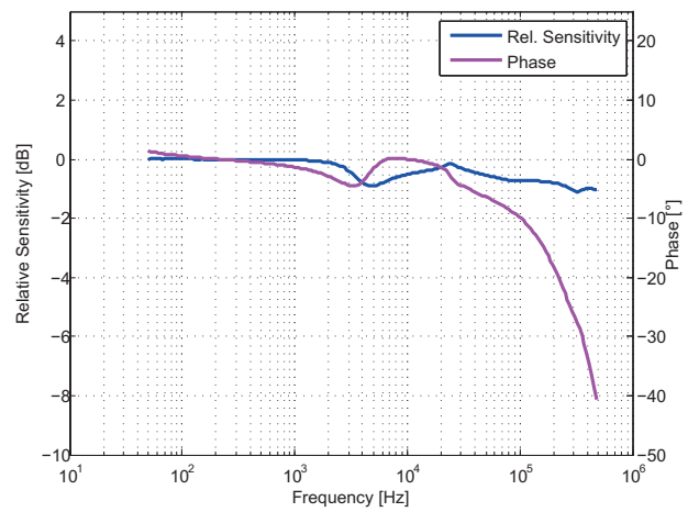
Figure 2: Frequency response
