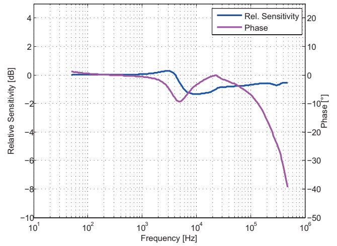
Figure 7: Frequency response
