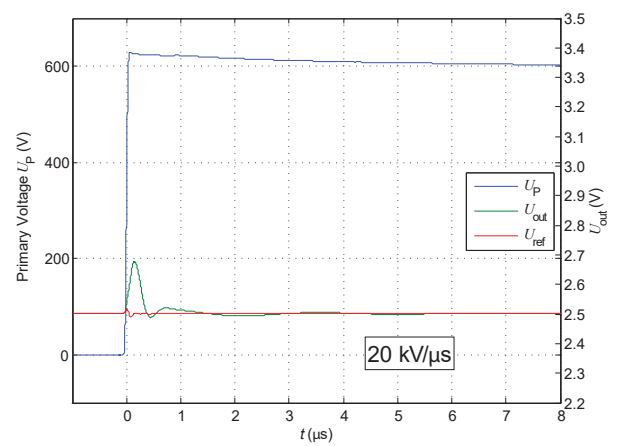
Figure 10: du/dt
