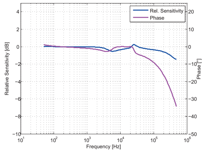
Figure 17: Frequency response
