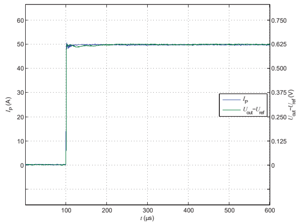
Figure 18: Delay time
