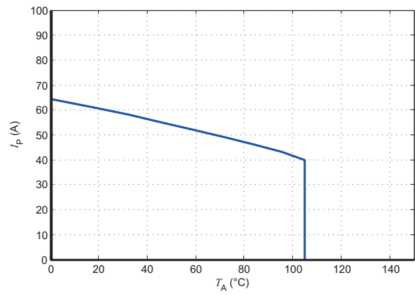
Figure 22: I_p vs T_A for LPSR 15-NP
