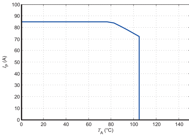
Figure 23: I_p vs T_A for LPSR 25-NP
