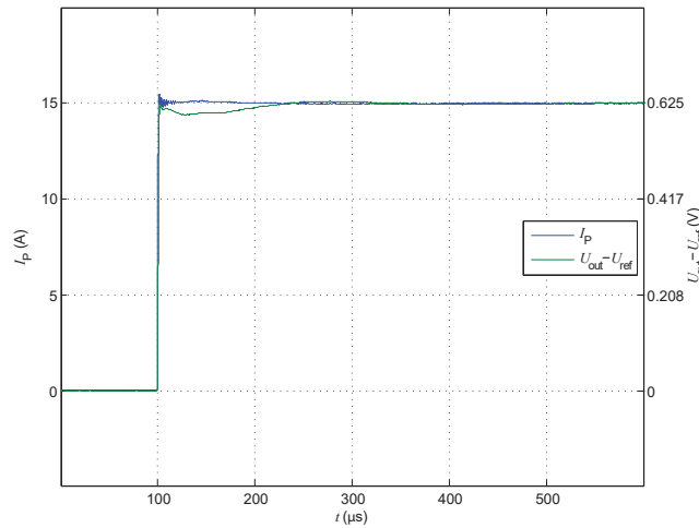
Figure 8: Delay time
