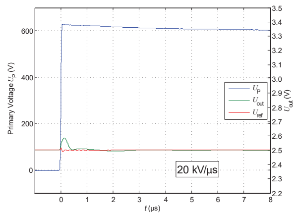
Figure 15: du/dt
