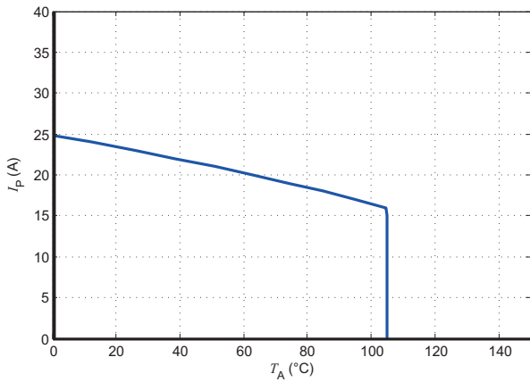
Figure 21: I_p vs T_A for LPSR 6-NP
