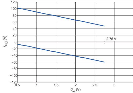
Figure 31: Measuring range versus external U_{ref} LPSR 15 A
