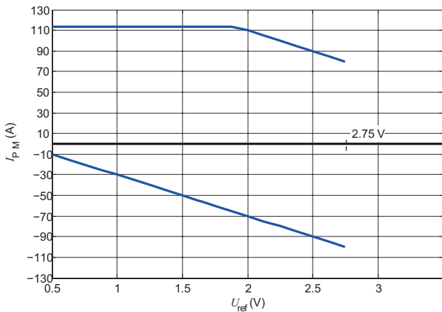
Figure 32: Measuring range versus external U_{ref} LPSR 25 A
