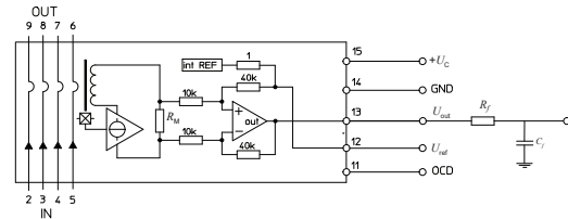
Figure 29: Filtered U_{out} connection
