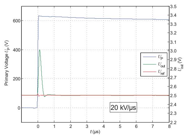
Figure 5: du/dt
