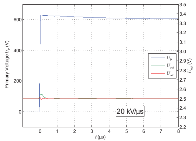
Figure 20: du/dt
