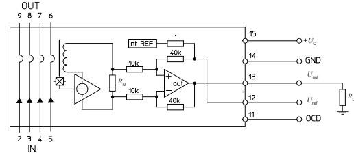
Figure 26: Test connection
