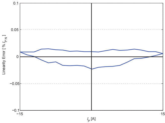
Figure 6: Linearity error
