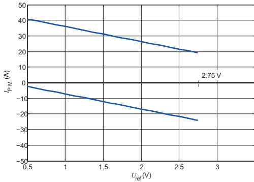
Figure 30: Measuring range versus external U_{ref} LPSR 6 A
