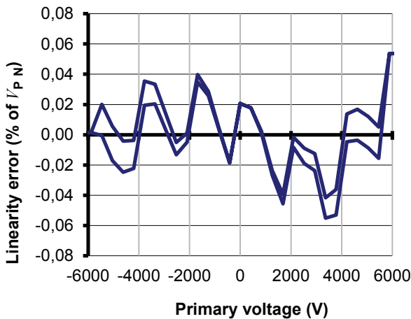
Figure 13: Typical linearity error at 25 °C
