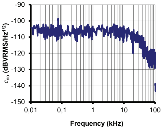
Figure 11: : Typical noise voltage density e_{no} with R_M = 50 \Omega
