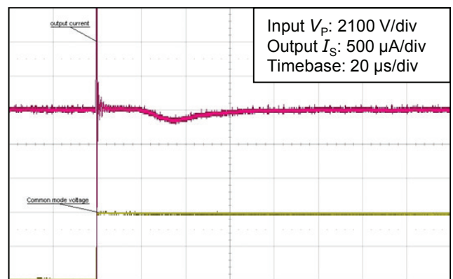
Figure 6: Detail of typical common mode perturbation (4200 V step with 6 kV/µs, R_M = 100 \Omega )
