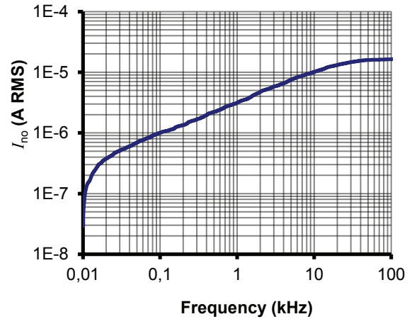
Figure 12: Typical total output RMS noise current with R_M = 50 \Omega
