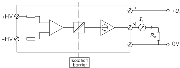
Figure 14: standard characterization schematics for current output transducers ( R_M = 50 \Omega unless otherwise noted)
