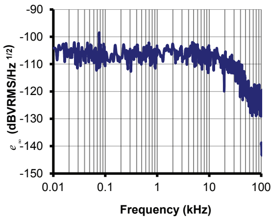
Figure 12: Typical noise voltage spectral density e_n with R_M = 50 \Omega
