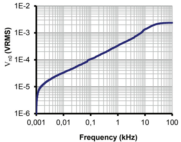
Figure 11: Typical total output RMS noise voltage spectral density V_{no} with R_M = 2 \text{ k}\Omega
