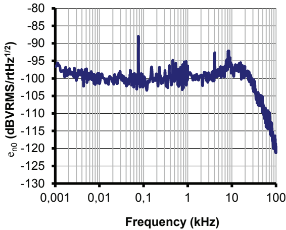
Figure 10: Typical total output RMS noise voltage spectral density e_{no} with R_M = 2 \text{ k}\Omega
