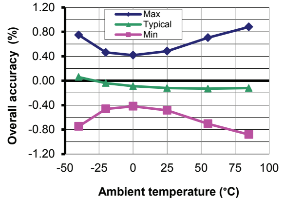
Figure 2: Overall accuracy in temperature
