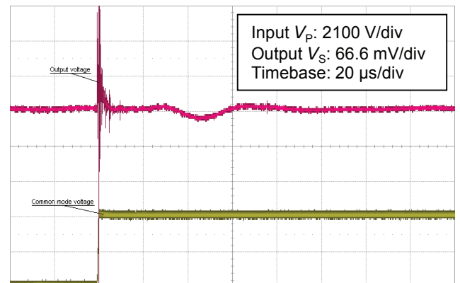
Figure 5: Detail of typical common mode perturbation (4200 V step with 6 kV/μs, RM = 2 kΩ)
