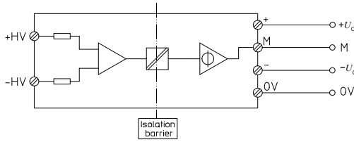
Figure 12: standard characterization schematics for voltage output transducers ( R_M = 2k\Omega unless otherwise noted)
