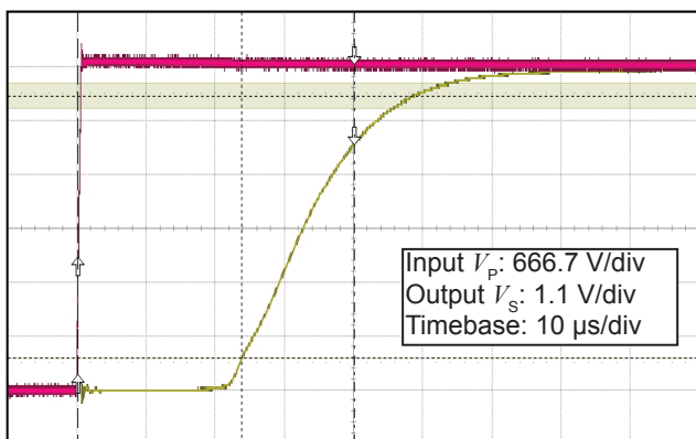
Figure 4: Typical step response (0 to 4000 V)
