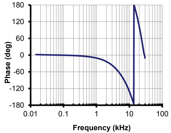
Figure Figure 9: Typical frequency and phase response
