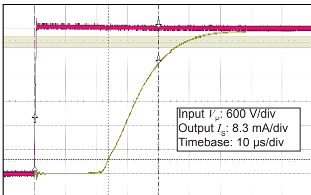
Figure 5: Typical step response (0 to 3600 V)
