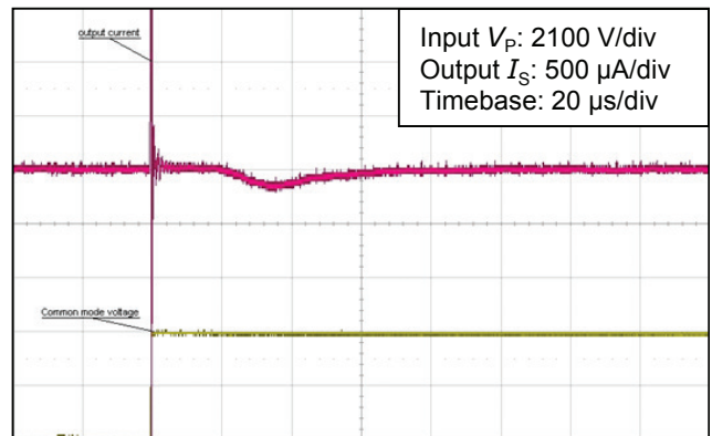
Figure 6: Detail of typical common mode perturbation (4200 V step with 6 kV/µs, RM = 100 Ω)
