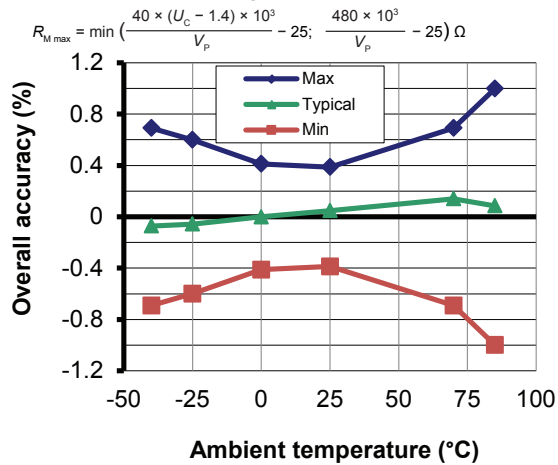
Figure 3: Overall accuracy in temperature
