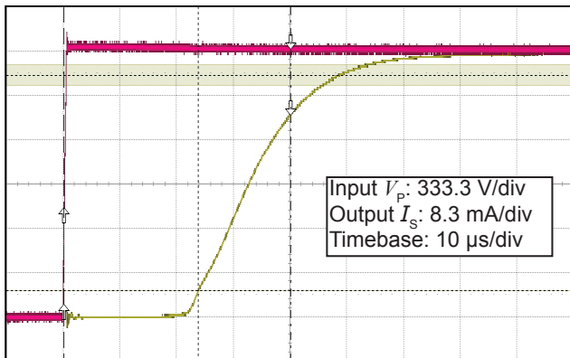
Figure 5: Typical step response (0 to 2000 V)
