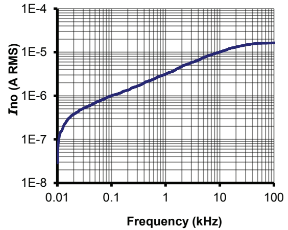
Figure 12: Typical total output RMS noise current with R_M = 100 \Omega
