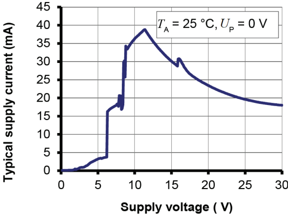
Figure 5: Supply current function of supply voltage
