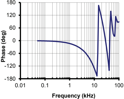
Figures 7 and 8: Typical frequency and phase response
