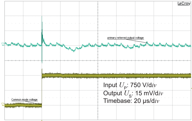
Figure 12: Detail of typical common mode perturbation (1500 V step with 6 kV/μs, R_M = 100 \text{ k}\Omega )
