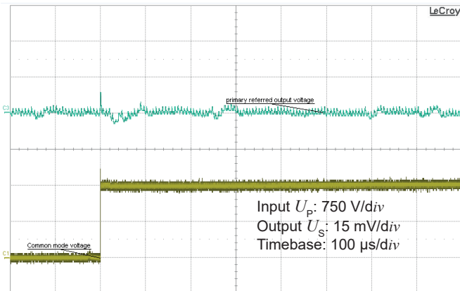
Figure 11: Typical common mode perturbation (1500 V step with 6 kV/μs, R_M = 100 \text{ k}\Omega )
