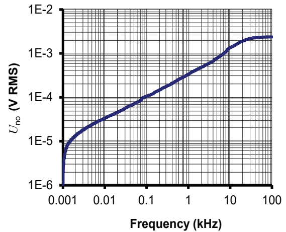
Figure 14: Typical total RMS noise voltage with R_M = 2 \text{ k}\Omega ( f_c is upper cut-off frequency of bandpass, low cut off frequency is 1 Hz)
