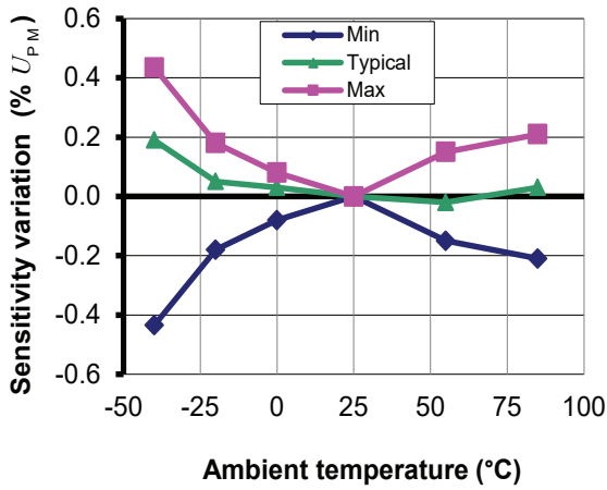
Figure 3: Sensitivity thermal variation
