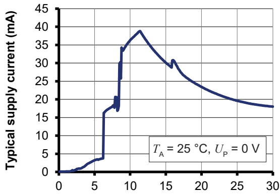
Figure 7: Supply current function of supply voltage
