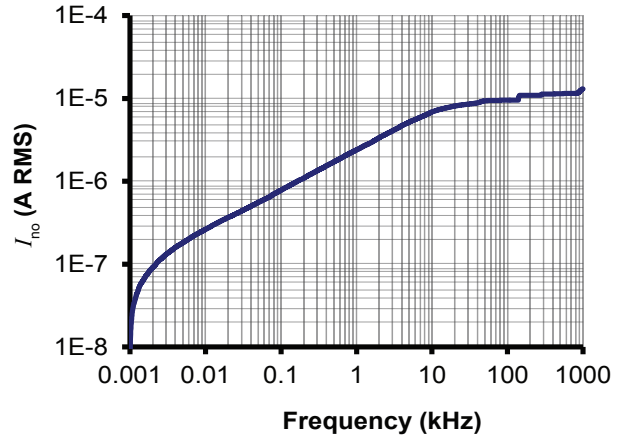
Figure 16: Typical total RMS noise current with R_M = 50 \Omega
