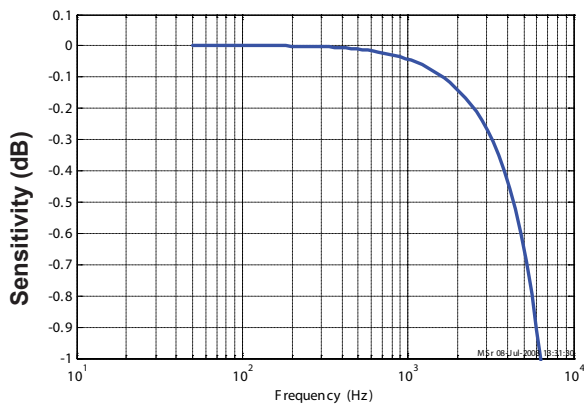
Figure 10 and 11: Typical frequency response (detail)
