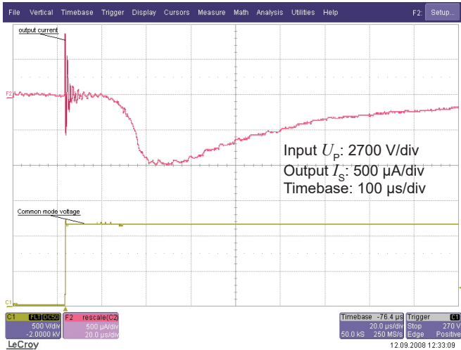
Figure 12: Typical common mode perturbation (6400 V step with 6 kV/μs, R M = 100 Ω)
