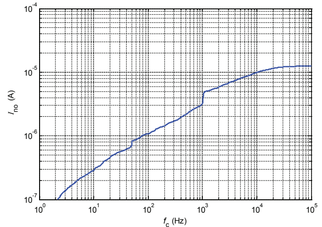
Figure 15: Typical total RMS noise current with R M = 50 Ω (f c is upper cut off frequency of band pass, low cut off frequency is 1 Hz)
