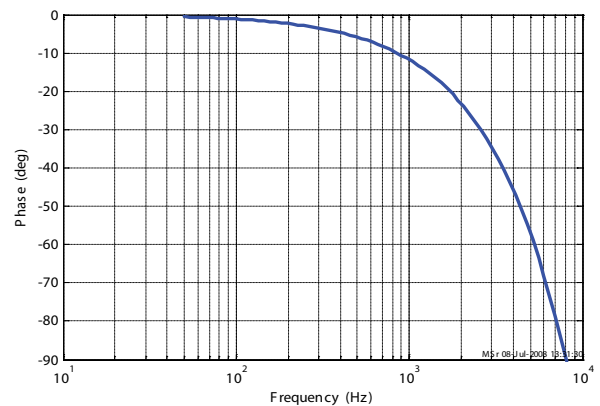
Figure 10 and 11: Typical frequency response (detail)
