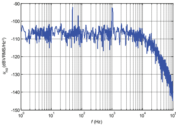
Figure 14: Typical noise voltage spectral density referred to primary with R M = 50 Ω
