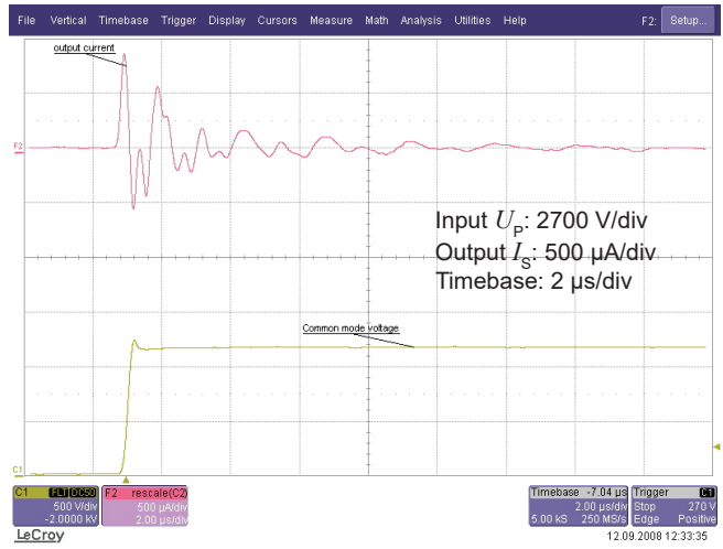
Figure 13: Detail of typical common mode perturbation (6400 V step with 6 kV/μs, R M = 100 Ω)
