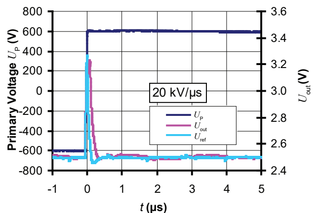
Figure 10: Step response
