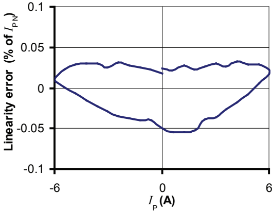
Figure 1: Linearity error
