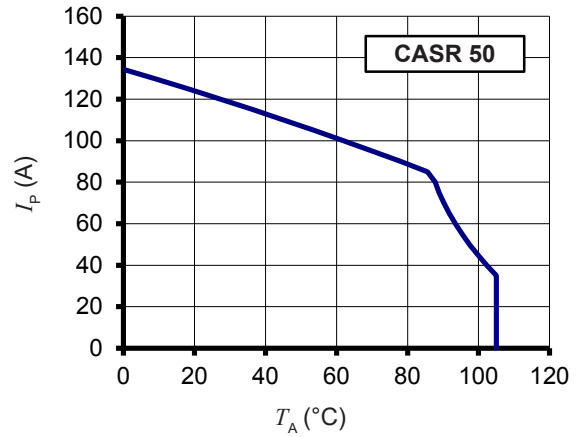
Figure 28: I_p vs T_A for CASR 50-NP/SP6
