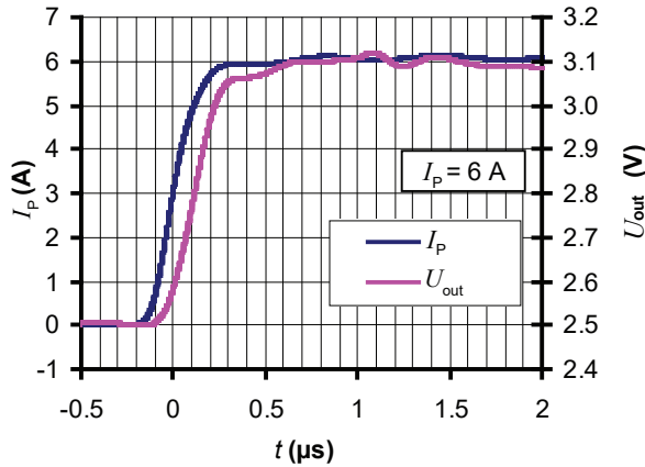
Figure 3: Step response
