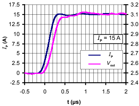
Figure 9: Step response
