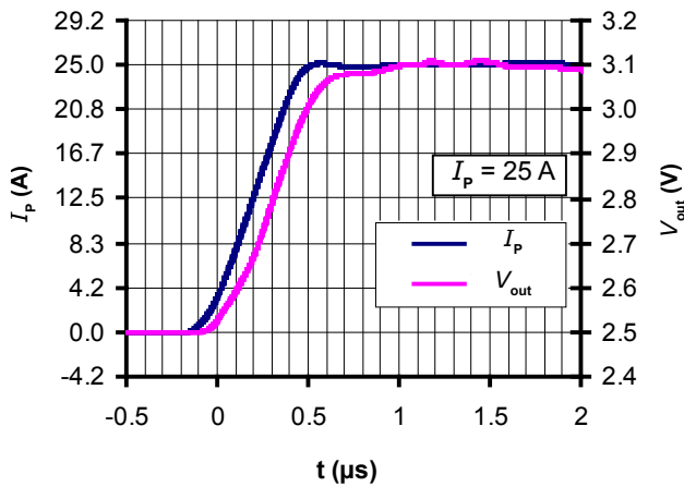
Figure 15: Step response
