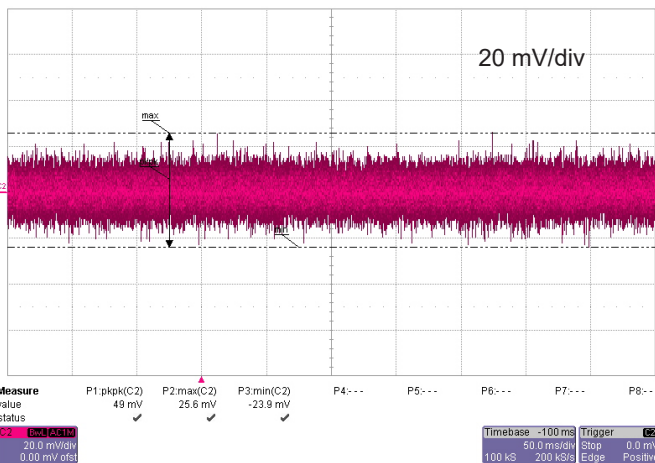
Figure 5: Output noise
