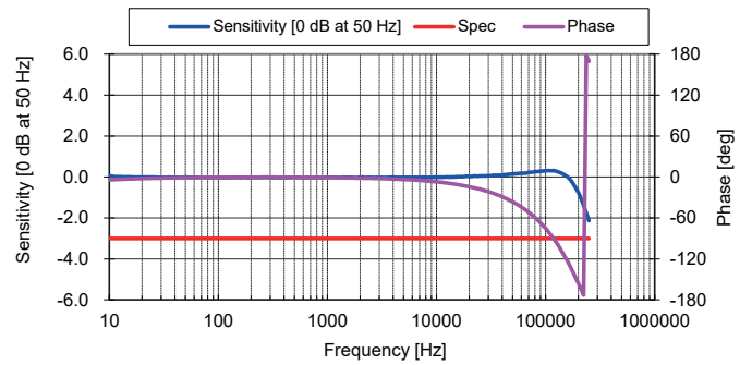
Figure 7: Frequency response
