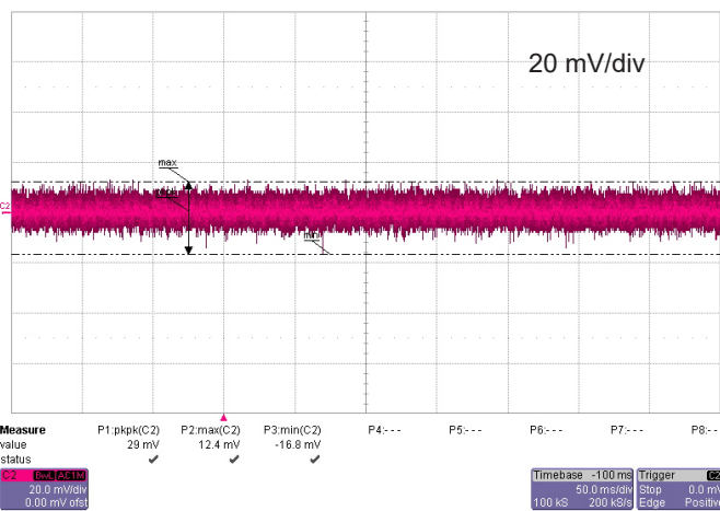
Figure 10: Output noise
