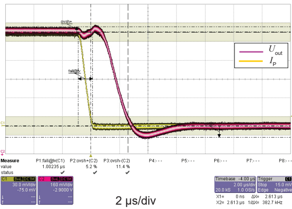
Figure 8: Step response
