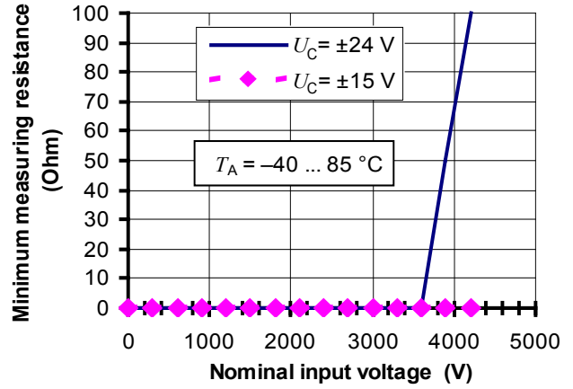
Figure 2: Minimum measuring resistance For T_A under 80 °C, the minimum measuring resistance is 0 Ω whatever U_C
