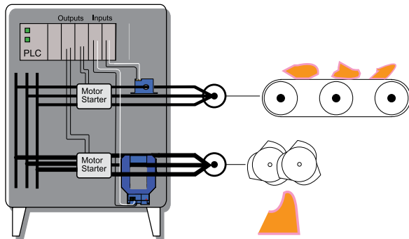
Grinder/Shredder Application
