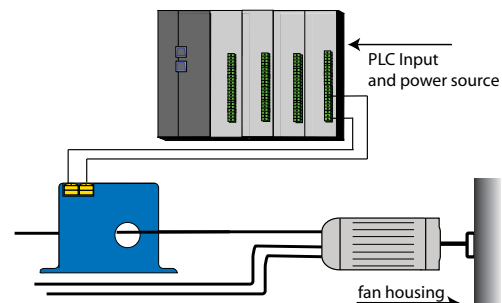
Current Sensing Switch Monitoring a Fan Load
