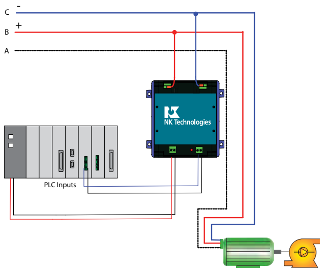
VTU Measures Both AC and DC Voltages
